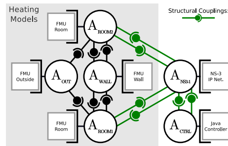
Figure 10. MECSYCO meta-model with only one IP model.
