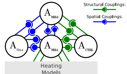
Figure 16. MECSYCO multi-model with three IP models (without model artifacts and models for readability).
