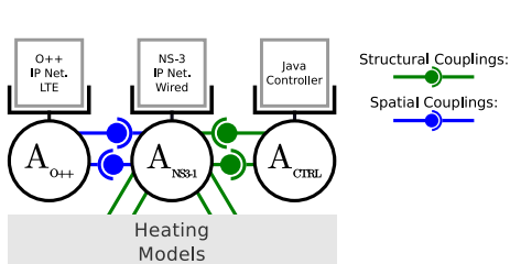
Figure 13. MECSYCO multi-model with two IP models.
