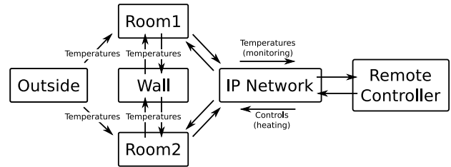
Figure 8. Intuitive graphic of the multi-model to compose.
